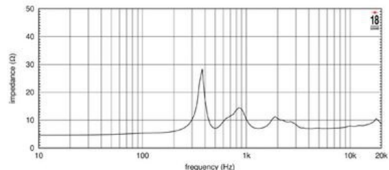
FREQUENCY RESPONSE MEASURED WITH 77.5 mV INPUT ON 2 in PLANE WAVE TUBE. IMPEDANCE MEASURED ON SAME PLANE WAVE TUBE
